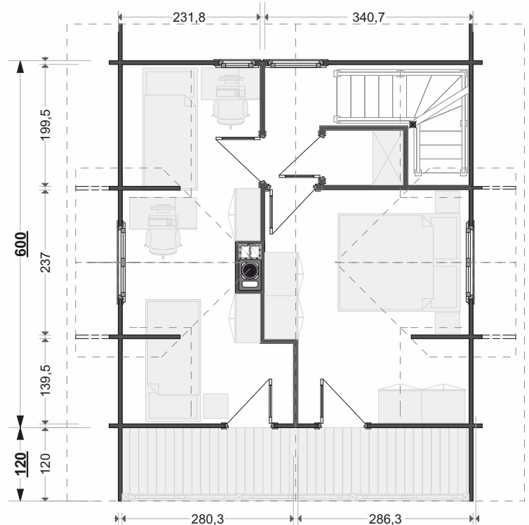
Poschodie / 1st floor
