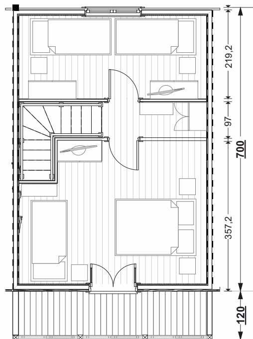
Poschodie/ 1st floor
